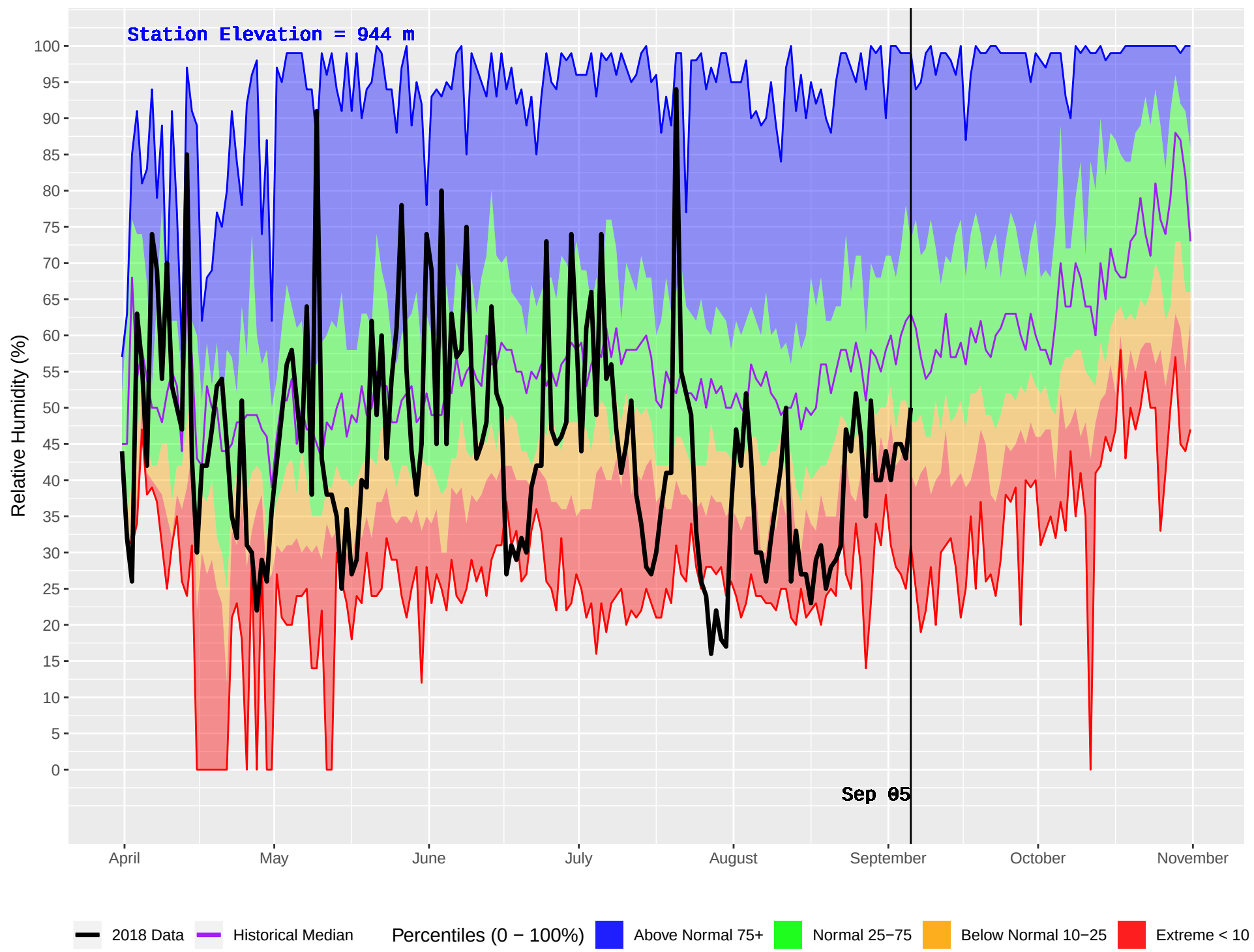
GRASSY PLAINS HUB (161) : Historical (1970–2016) and Current (2018) Daily Relative Humidity
